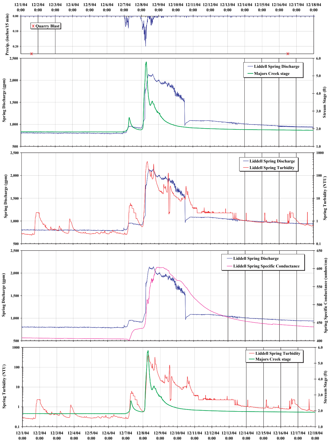
Storm Hydrograph Comparison, December 2004
